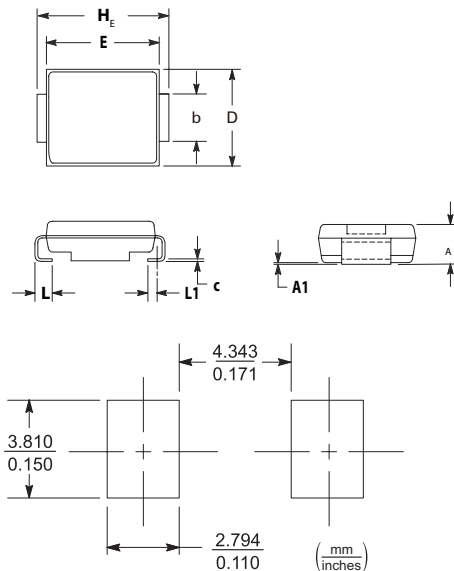
Soldering Footprint
