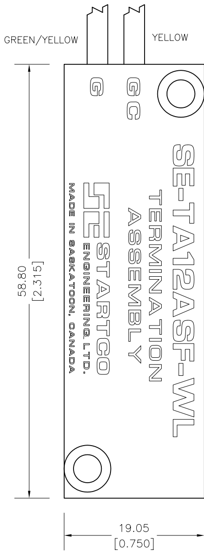
TOP VIEW
