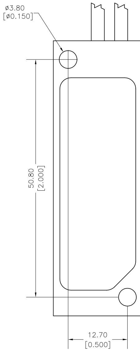
BOTTOM VIEW
