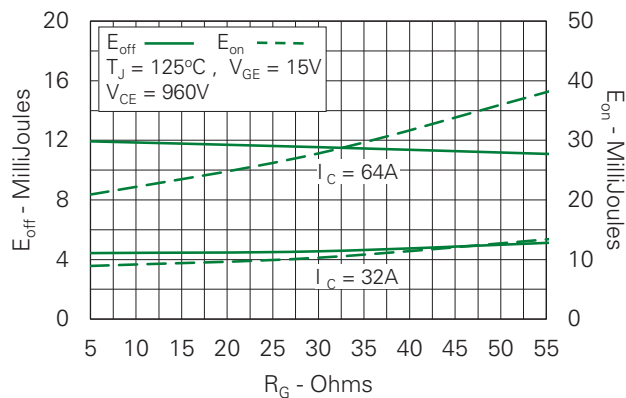
Fig. 12. Inductive Switching Energy Loss vs. Gate Resistance
