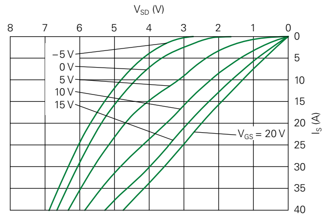
Fig. 6. Typical Reverse Conduction Characteristics ( T_{VJ} = 25\text{ }^{\circ}\text{C} )
