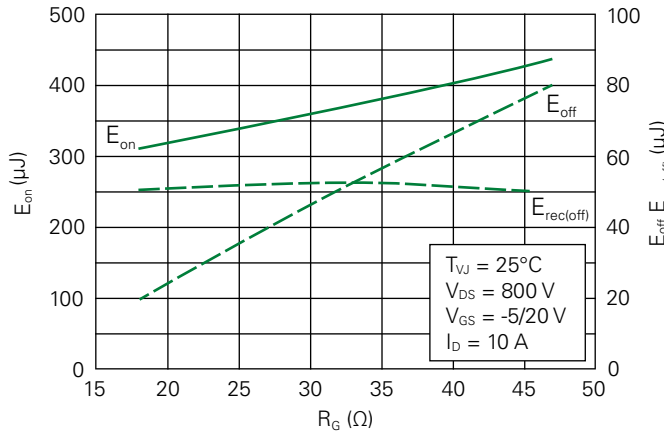
Fig. 19. Typical Switching Energy at 25 °C vs. External Gate Resistor
