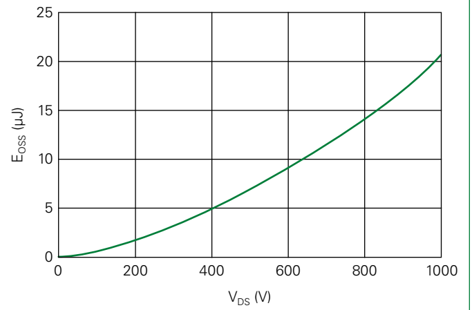
Fig. 16. Typical C_{OSS} Stored Energy E_{OSS}
