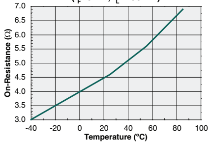
On-Resistance vs. Temperature DC-Only Configuration ( I_F=0mA , I_L=100mA )
