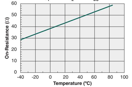
Typical On-Resistance vs. Temperature ( I_F=5mA, I_L=50mA_{DC} )
