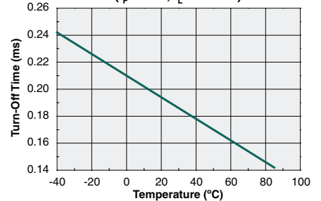
Typical Turn-Off Time vs. Temperature ( I_F=5\text{mA} , I_L=100\text{mA} )
