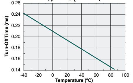
Typical Turn-Off Time vs. Temperature ( I_F=5\text{mA} , I_L=100\text{mA} )
