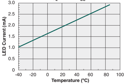
Typical I_F for Switch Operation vs. Temperature ( I_L=200\text{mA}_{\text{DC}} )
