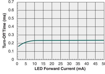
Typical Turn-Off Time vs. LED Forward Current ( I_L=50mA_{DC} )
