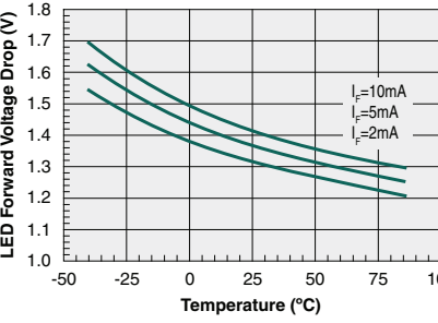
Typical LED Forward Voltage Drop vs. Temperature
