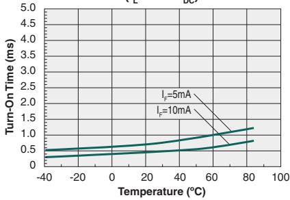
Typical Turn-On Time vs. Temperature ( I_L = 50 \text{ mA}_{DC} )
