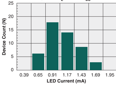
Typical I_F for Switch Dropout (N=50, I_L=120mA_{DC} )
