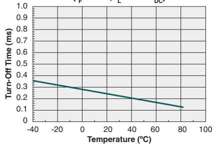
Typical Turn-Off Time vs. Temperature ( I_F = 5 \text{ mA} , I_L = 50 \text{ mA}_{DC} )
