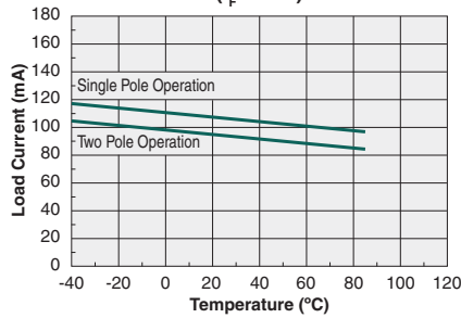
Maximum Load Current vs. Temperature ( I_F = 5 \text{ mA} )
