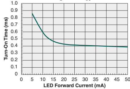
Typical Turn-On Time vs. LED Forward Current ( I_L=250mA_{DC} )
