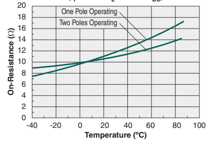
Typical On-Resistance vs. Temperature ( I_F=5\text{mA} , I_L=200\text{mA}_{DC} )
