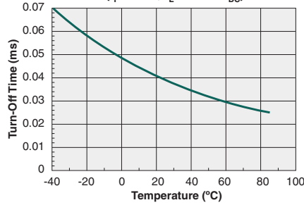
Typical Turn-Off Time vs. Temperature ( I_F=5\text{mA}, I_L=250\text{mA}_{DC} )
