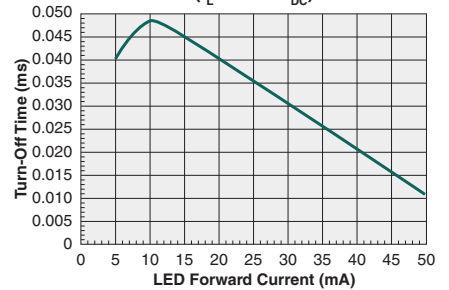
Typical Turn-Off Time vs. LED Forward Current ( I_L=250mA_{DC} )
