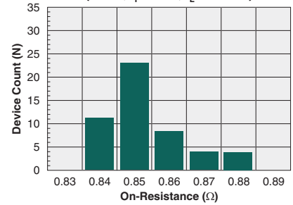
Typical On-Resistance Distribution (N=50, I_F=5\text{mA} , I_L=600\text{mA} )
