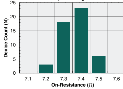
Typical On-Resistance Distribution ( N=50, I_F=3mA, I_L=200mA )
