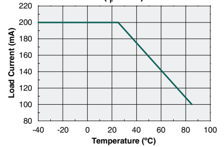
Maximum Load Current vs. Temperature ( I_F=3\text{mA} )
