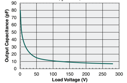
Output Capacitance vs. Load Voltage ( I_F=0\text{mA} )
