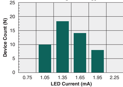
Typical I_F for Switch Operation (N=50, I_L=150mA_{DC} )
