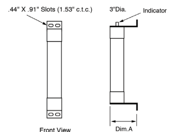
Bolt-In Mount "BI"
