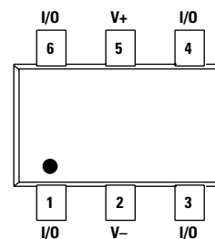
SP724 (SOT-23) TOP VIEW
