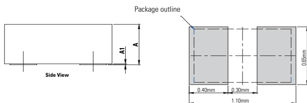
Recommended soldering pad layout
