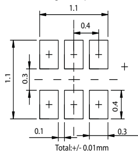
Recommended Soldering Pad for μDFN-6L 1.25 x1.0x0.5 mm
