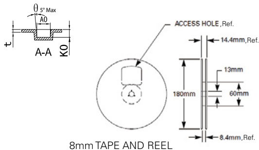
8mm TAPE AND REEL
