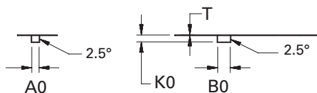
Component Orientation in Tape
