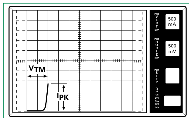
Figure AN1006.25 V_{TM(\text{Forward})} = 950 \text{ mV} at I_{PK} = 1.4 \text{ A}
