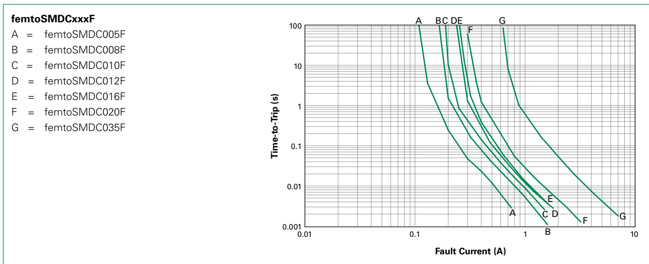
Typical Time-to-Trip Curves at 20°C
