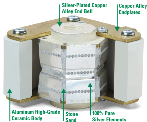
Figure 10: Square Body Style Fuses
