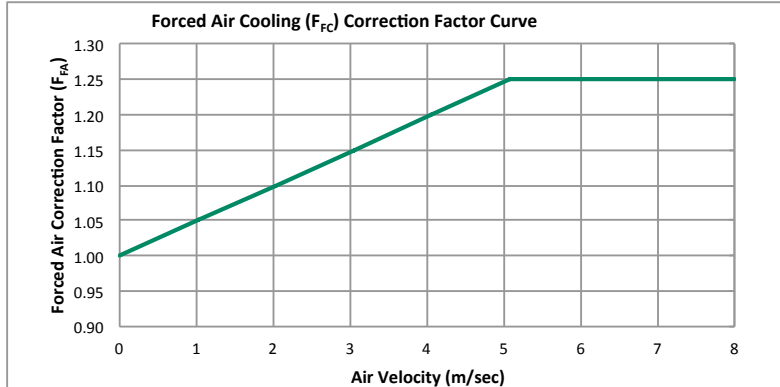
Figure 30: Forced (Air) Cooling Correction Factor ( F_{FC} ) Curve
