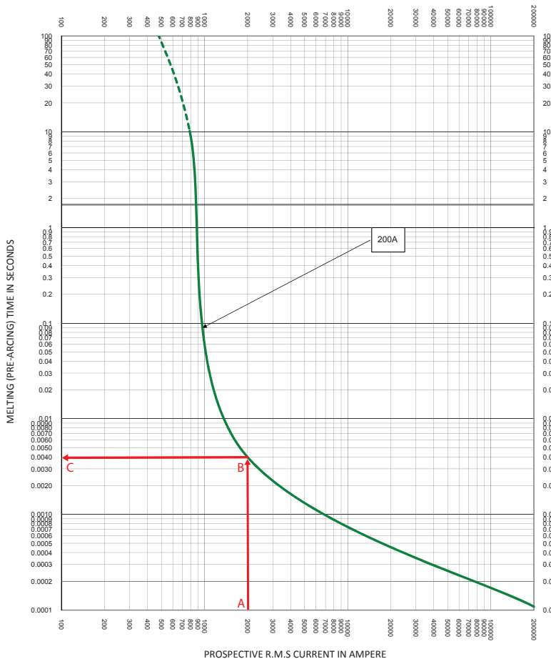
Figure 14: Time Current Characteristic Curve – Pre-arcing (Melting) Time determination
