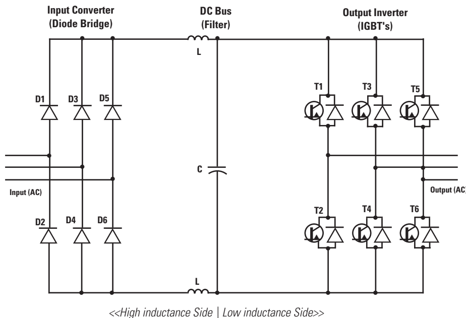
Figure 37: Typical Three Phase Power Converter Circuit
