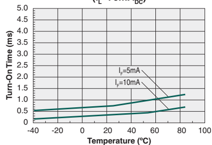
Typical Turn-On Time vs. Temperature ( I_L = 70\text{mA}_{\text{DC}} )
