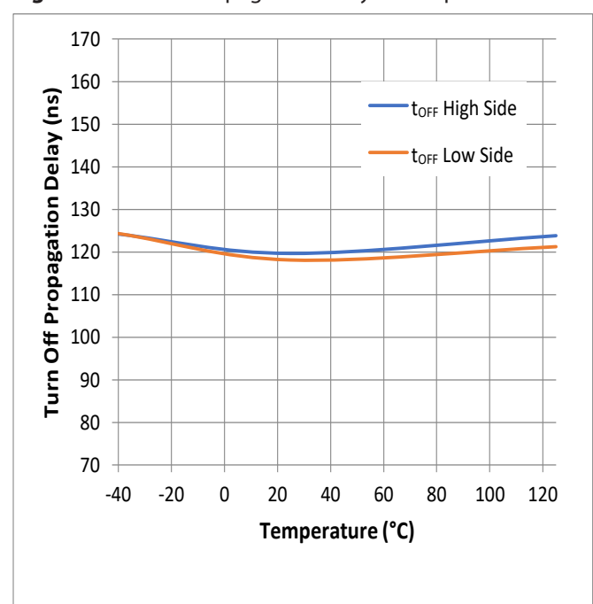
Figure 7. Turn Off Propagation delay vs Temperature
