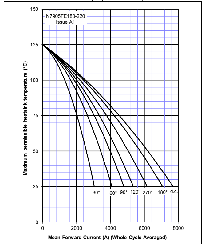
Figure 16 – On-state current vs. Heatsink temperature – Cathode Side Cooled (Square wave)
