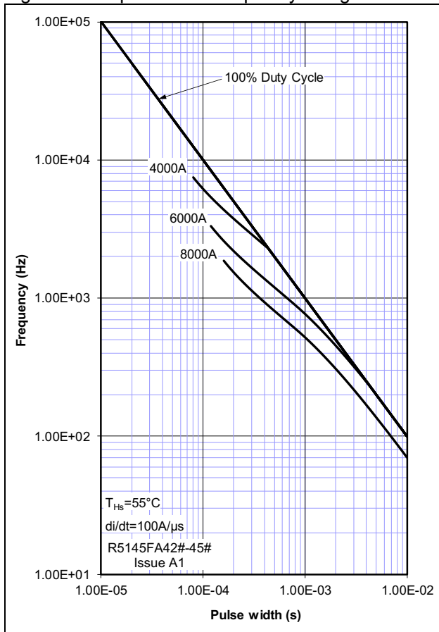
Figure 13 - Square wave frequency ratings
