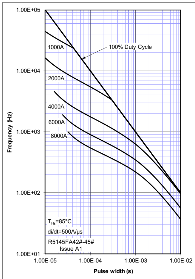
Figure 16 - Square wave frequency ratings
