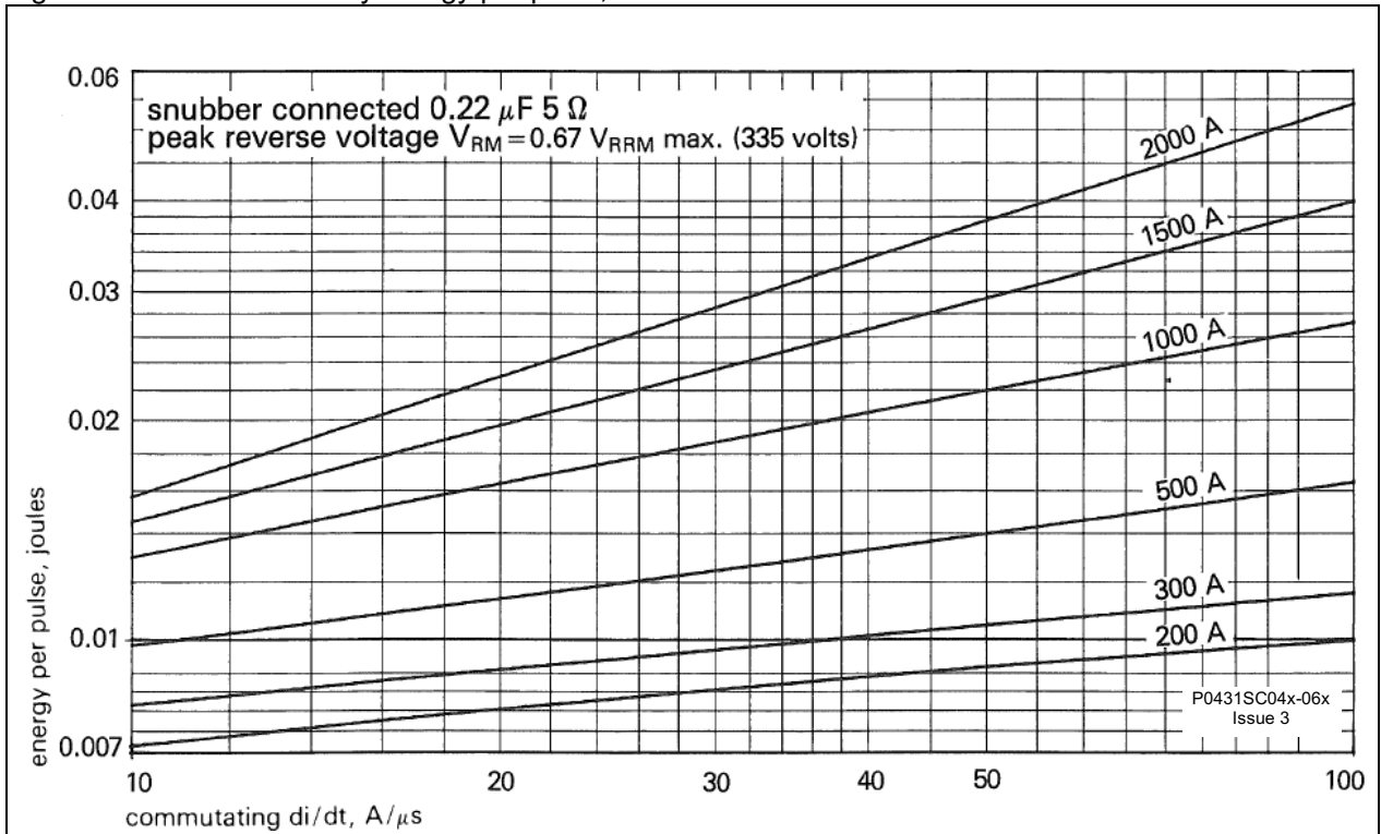
Figure 4 – Reverse recovery energy per pulse, E_{rm}
