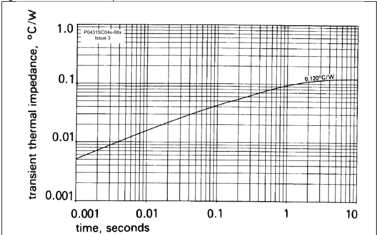
Figure 3 – Transient thermal impedance R_{thJK}
