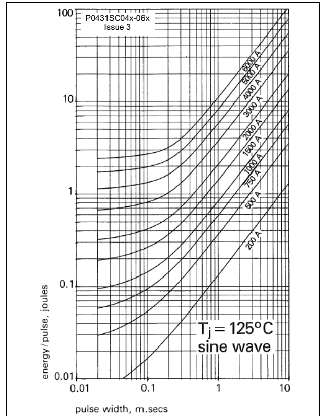
Figure 6 - Sine wave energy per pulse
