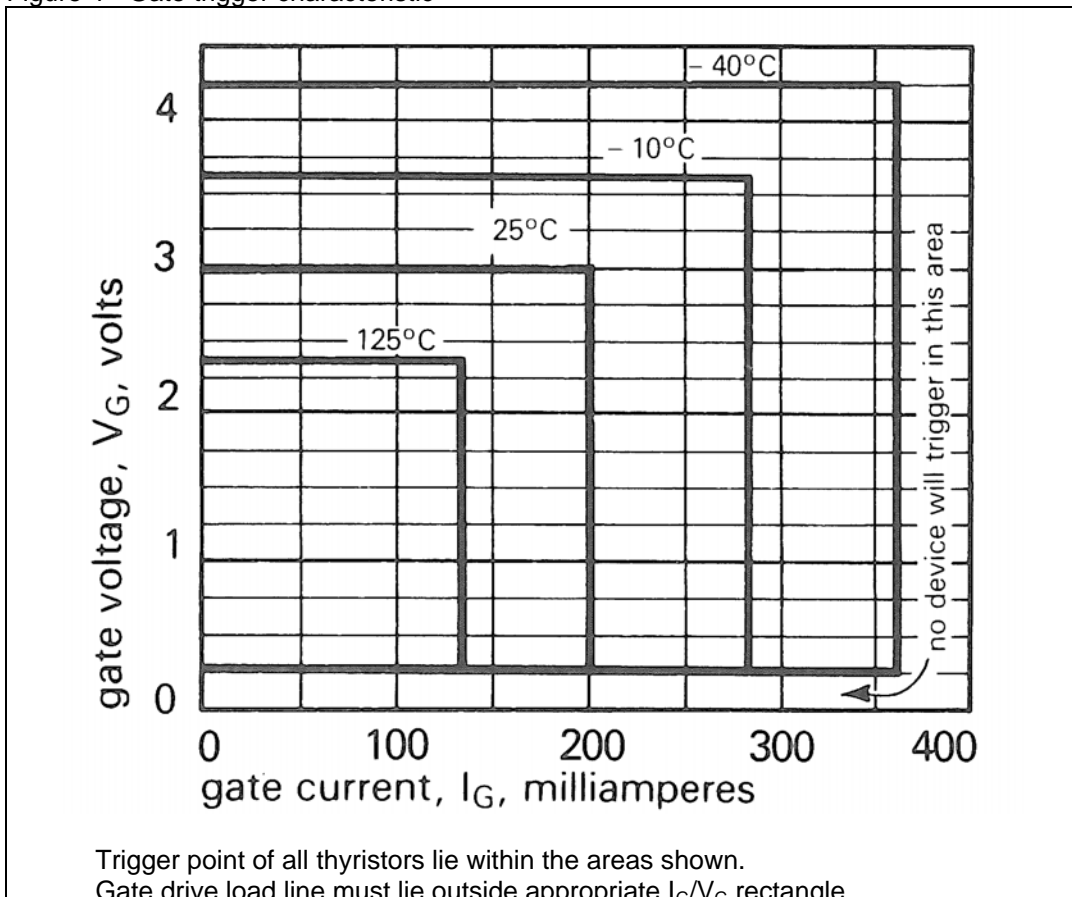
Figure 4 - Gate trigger characteristic
