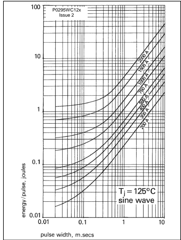
Figure 6 - Sine wave energy per pulse
