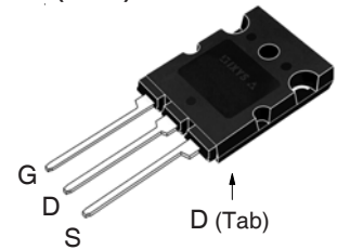
TO-264 (IXFK)
