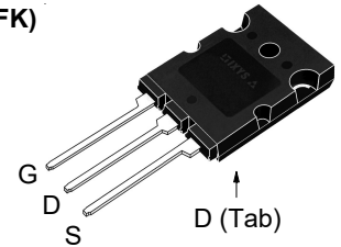
TO-264K (IXFK)
