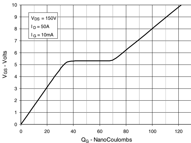
Fig. 11. Gate Charge
