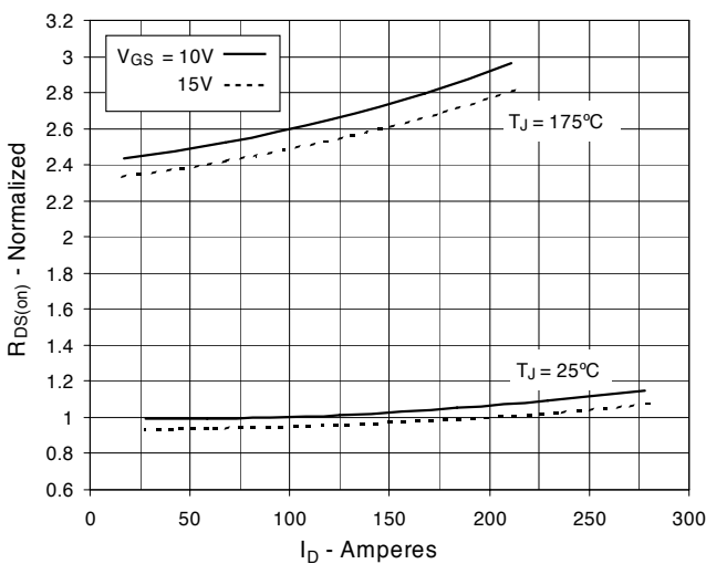
Fig. 5. R_{DS(on)} Normalized to I_D = 80A Value vs. Drain Current
