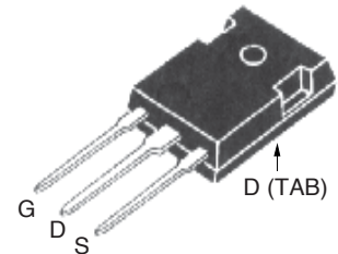
TO-3P (IXTQ)
