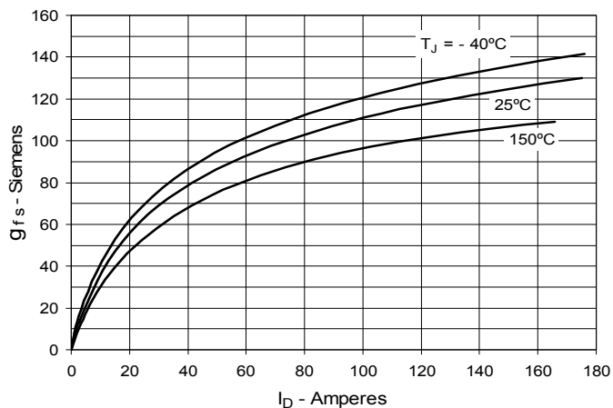
Fig. 8. Transconductance
