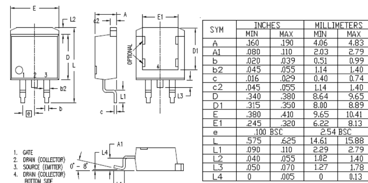
TO-263 (IXTA) Outline
