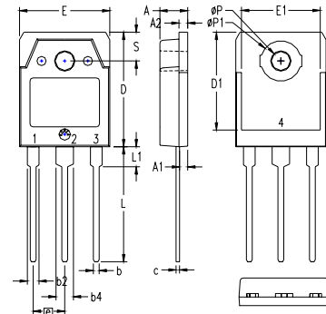
TO-3P (IXTQ) Outline
