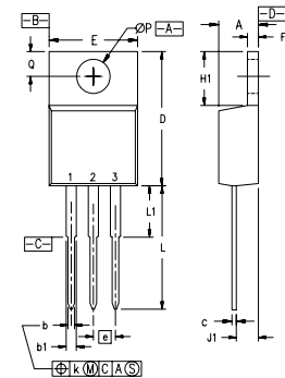
TO-220 (IXTP) Outline
