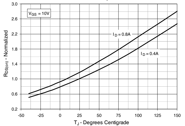
Fig. 4. R_{DS(on)} Normalized to I_D = 0.4A Value vs. Junction Temperature
