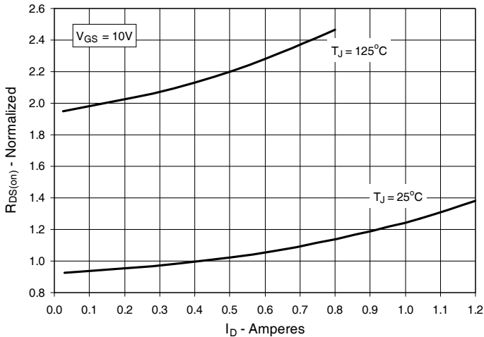
Fig. 5. R_{DS(on)} Normalized to I_D = 0.4A Value vs. Drain Current
