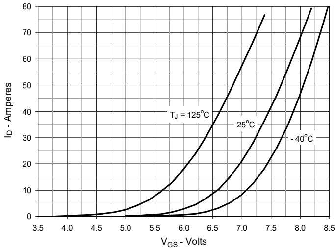
Fig. 7. Input Admittance
