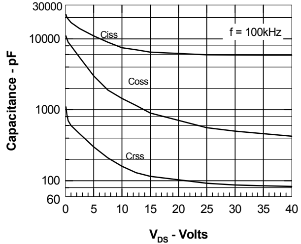
Fig. 8 Capacitance Curves
