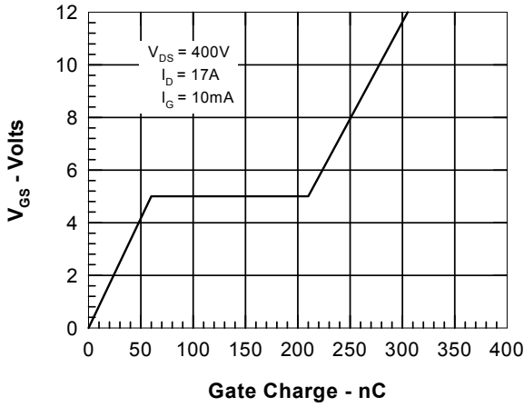
Figure 7. Gate Charge
