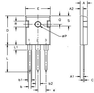
Terminals: 1 - Gate 2 - Drain 3 - Source TAB - Drain
