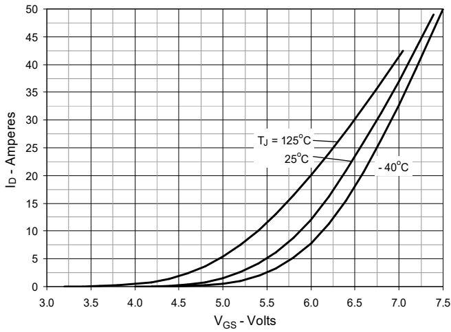
Fig. 7. Input Admittance
