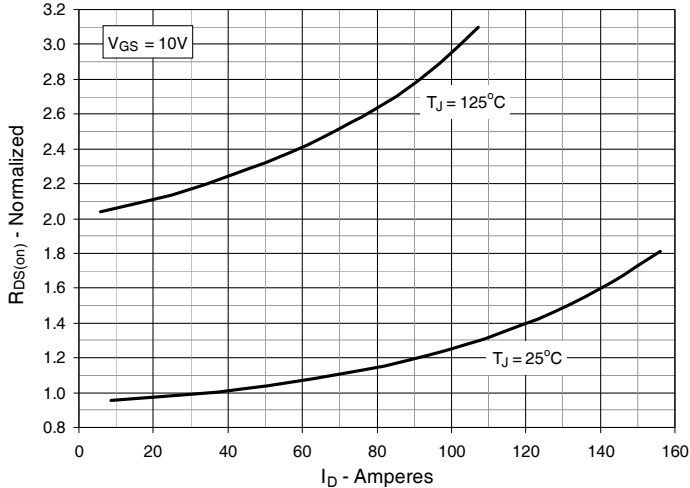
Fig. 5. R_{DS(on)} Normalized to I_D = 39A Value vs. Drain Current
