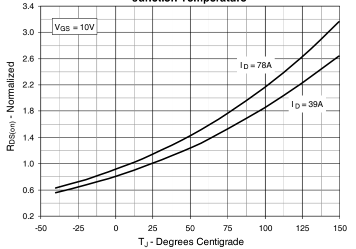
Fig. 4. R_{DS(on)} Normalized to I_D = 39A Value vs. Junction Temperature
