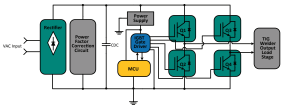
Figure 2: TIG Welding Inverter
