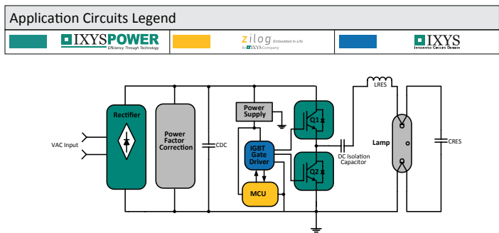
Figure 1: Electronic Lamp Ballast
