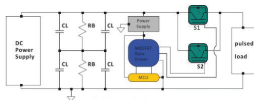
Figure 1: Pulse circuit
