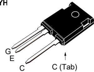
TO-247HV (IXYH)
